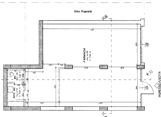
PIANO SEMINTERRATO Scala 1:50
